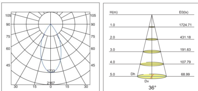
Typical light distribution for 4000K 36°
