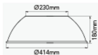
70° PC Diffuser
