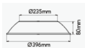
90° Aluminium Reflector
