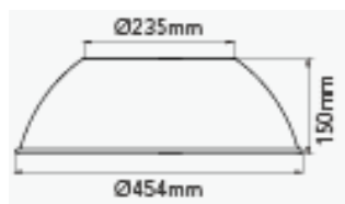
70° Aluminium Reflector
